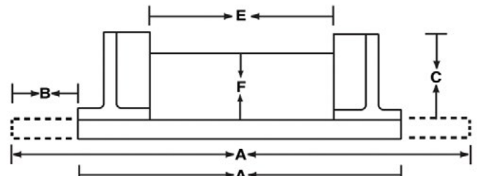
D - Example of Sidewall (foot out)
